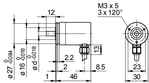
BMSV/BMMV 30R SSI, cable radial
