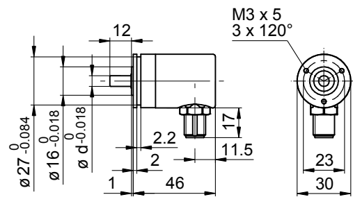
BMSV/BMMV 30R SSI, connector radial
